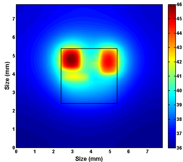
Figure 2: Temperature rise map for the layout from Figure 1.
