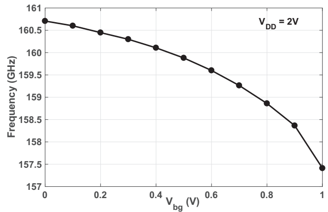
Fig. 9. Variation of oscillation frequency via back-gate bias around 160 \text{ GHz} .
