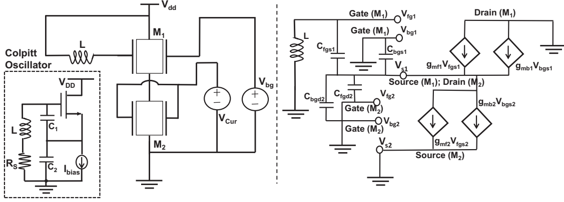
Fig. 2. The Colpitts oscillator designed utilizing the device parasitics and its small signal model.
