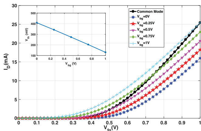
Fig. 1. I_D - V_{fg} characteristics of an n-type Independent ( V_{bg} \neq V_{fg} ) and Common ( V_{bg} = V_{fg} ) Mode DG transistors with BSIM-IMG FinFET. The inset shows the resulting shift in the front gate threshold.
