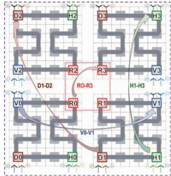
Fig. 12. 256-Core OWN architecture. Routers with same color communicate with each other [8].
