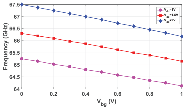
Fig. 6. Variation of oscillation frequency with different back gate bias at three different supply voltages at 60 GHz.
