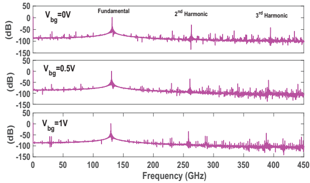
Fig. 11. The PSD of the DG-FinFET oscillator with higher order harmonics highlighted for future design of push-push oscillators to achieve oscillation frequency upto 400 GHz. The width considered here is 12 \mu\text{m} .
