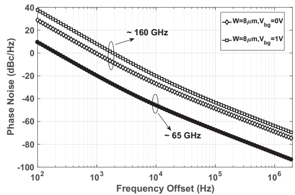
Fig. 10. The phase noise at the center frequency of 60 \text{ GHz} and 160 \text{ GHz} .
